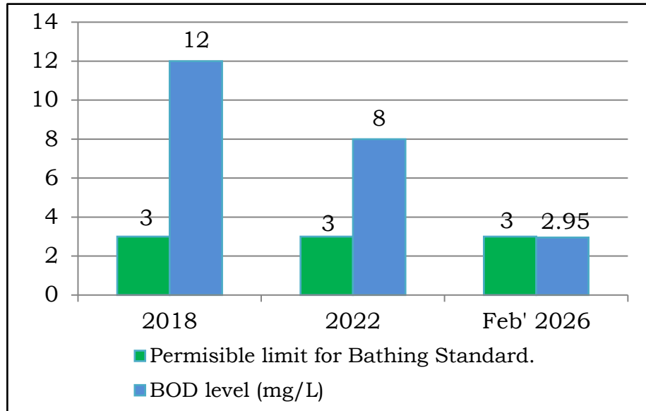
Comparative Analysis of BOD in River Ganga
